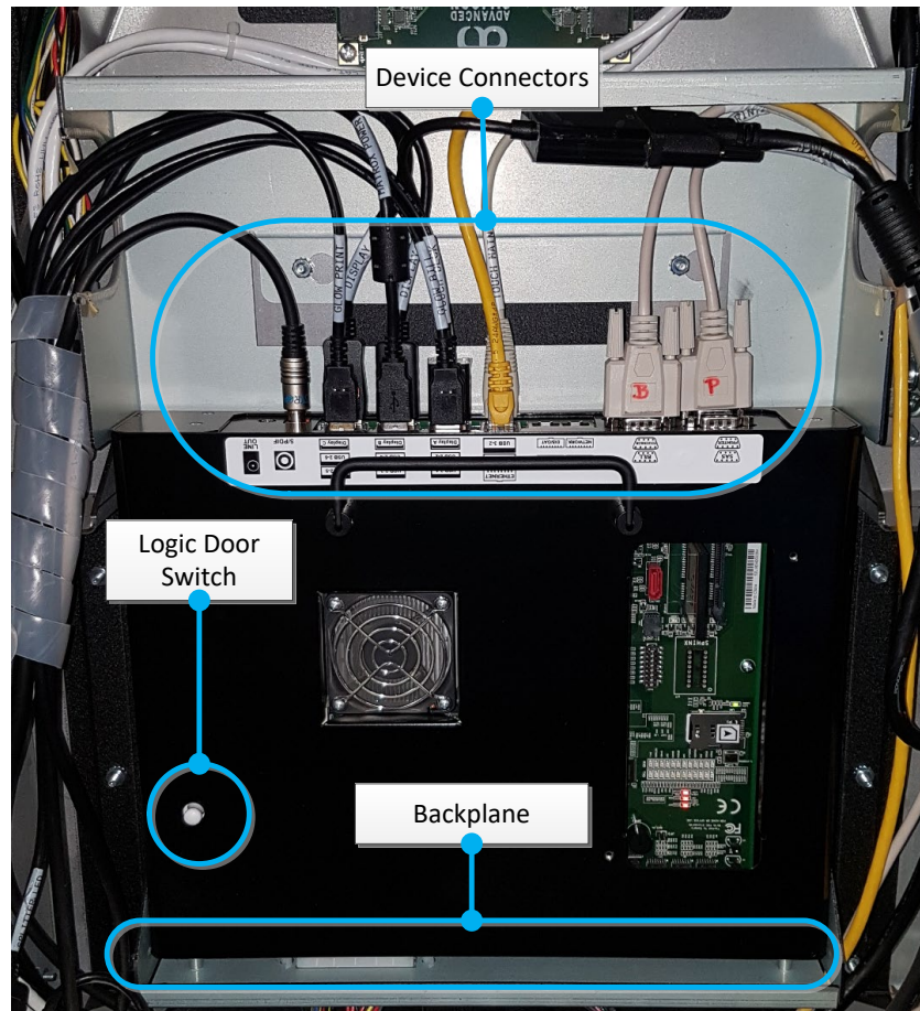
Logic Box Inside View
